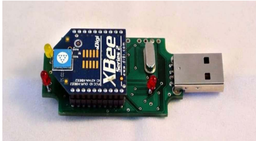
Fig.2. Sensor
